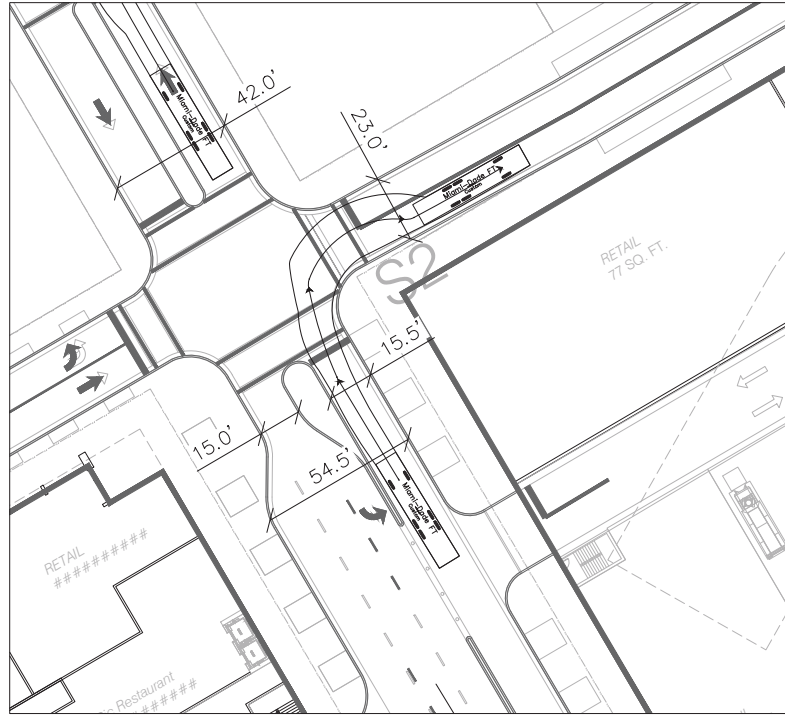
DETAIL I
