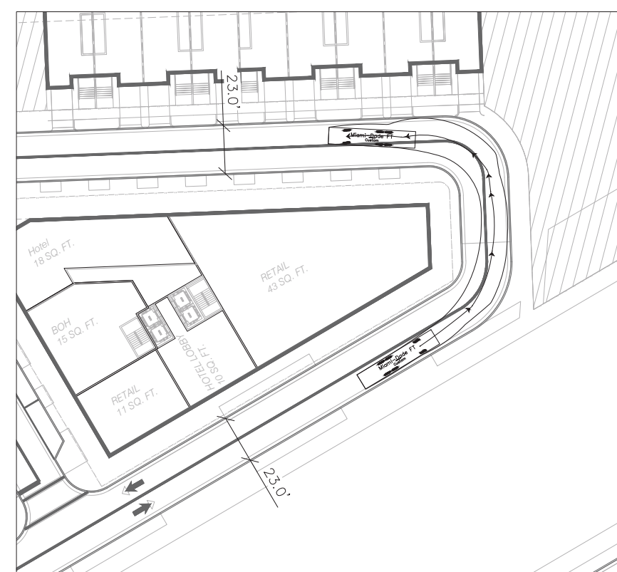
DETAIL B
