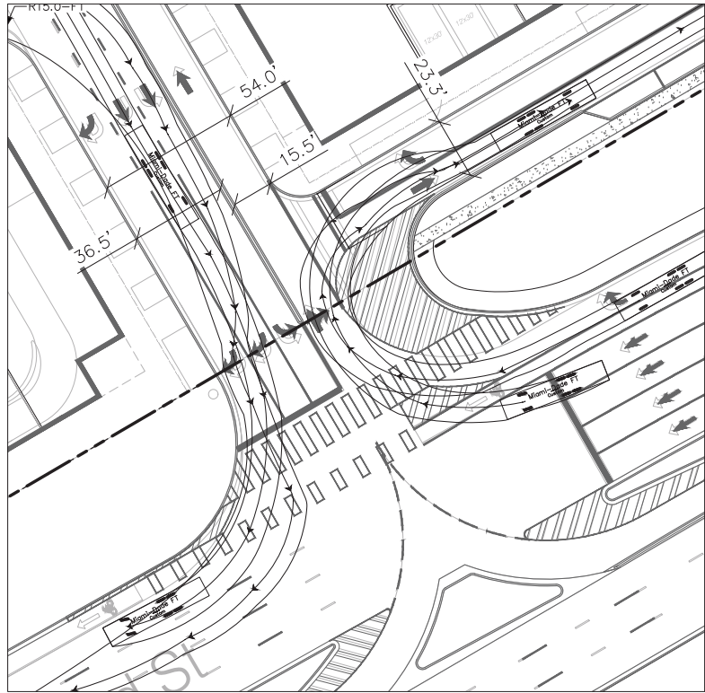
DETAIL H
