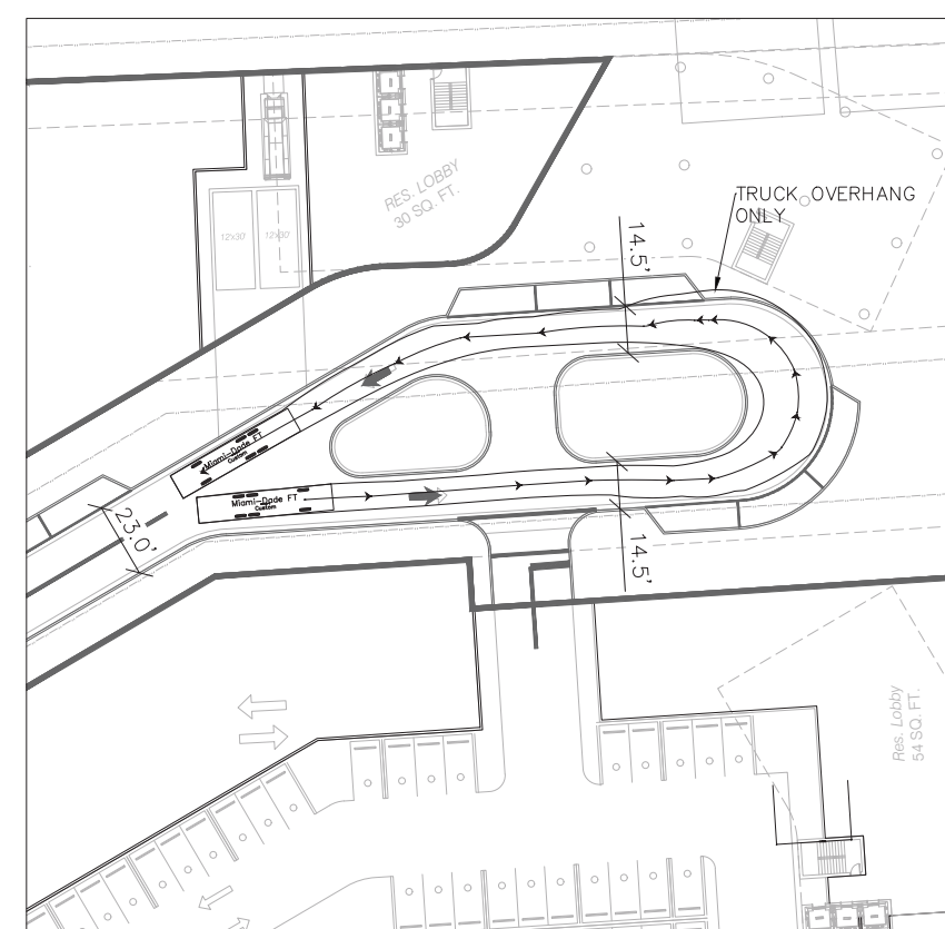
DETAIL C
