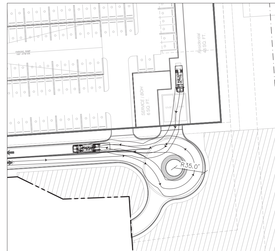
DETAIL J
