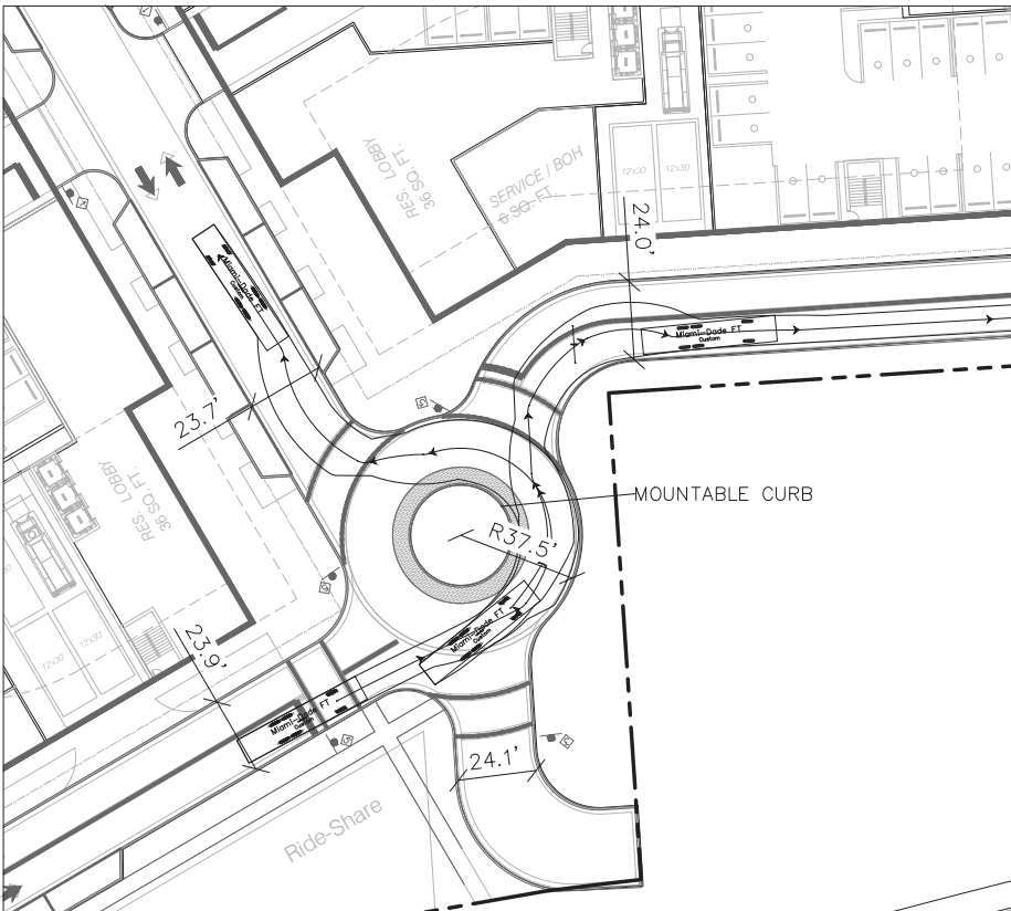
DETAIL F
