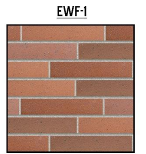
EWF-1 BELDEN NORMAN BRICK MASONRY MEDIUM RANGE, SMOOTH, IRON SPOT. MORTAR TO MATCH SOLOMON PRODUCTS IO H. WEATHERED HORIZONTAL STRIKE. VERTICAL JOINTS ARE FLUSH
